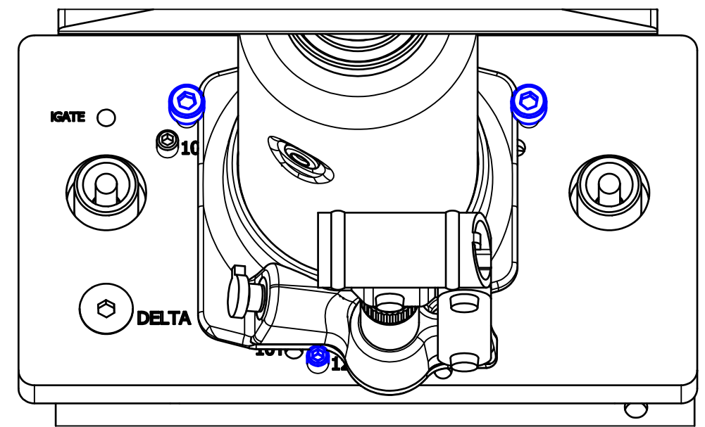
jacket plate shown in configuration for jack 12 ton
